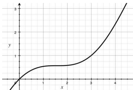
Figure 4. Graph representation of formula (2).
