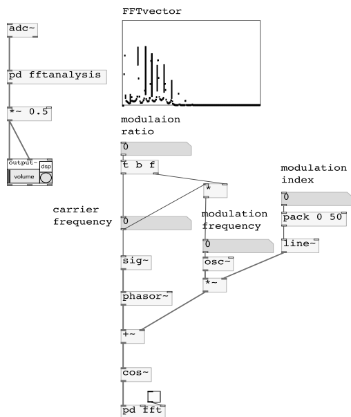
Figure 5. Pd-extended patch using FM synthesis to rewrite 256-bin FFT vectors controlling a spectral filter.
