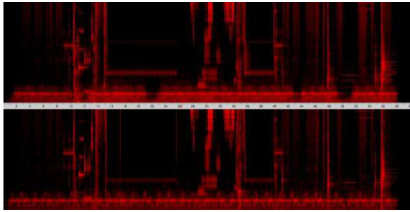
Figure 1. Sonogram analysis of the first minute of Parmegiani's "Points contre champs".
