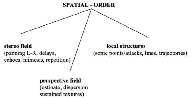
Figure 3. Spatial order in Parmegiani's "Points contre champs".
